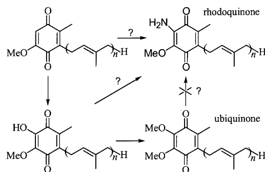
Figure 1. The last three steps of the ubiquinone biosynthesis in eukaryotic organisms, and the proposed precursors of rhodoquinone biosynthesis; in mammals and rats, n = 10 and n = 9 , respectively; in this paper systems with n = 2 have been prepared
